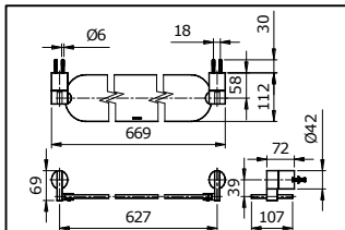
TX705AE "EGO" Glass Shelf (L= 669 mm)
