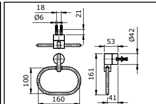
TX702AE "EGO" Towel Ring
