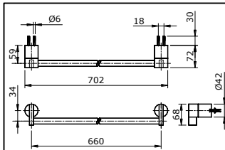
TX701AE "EGO" Towel Bar (L= 660 mm)
